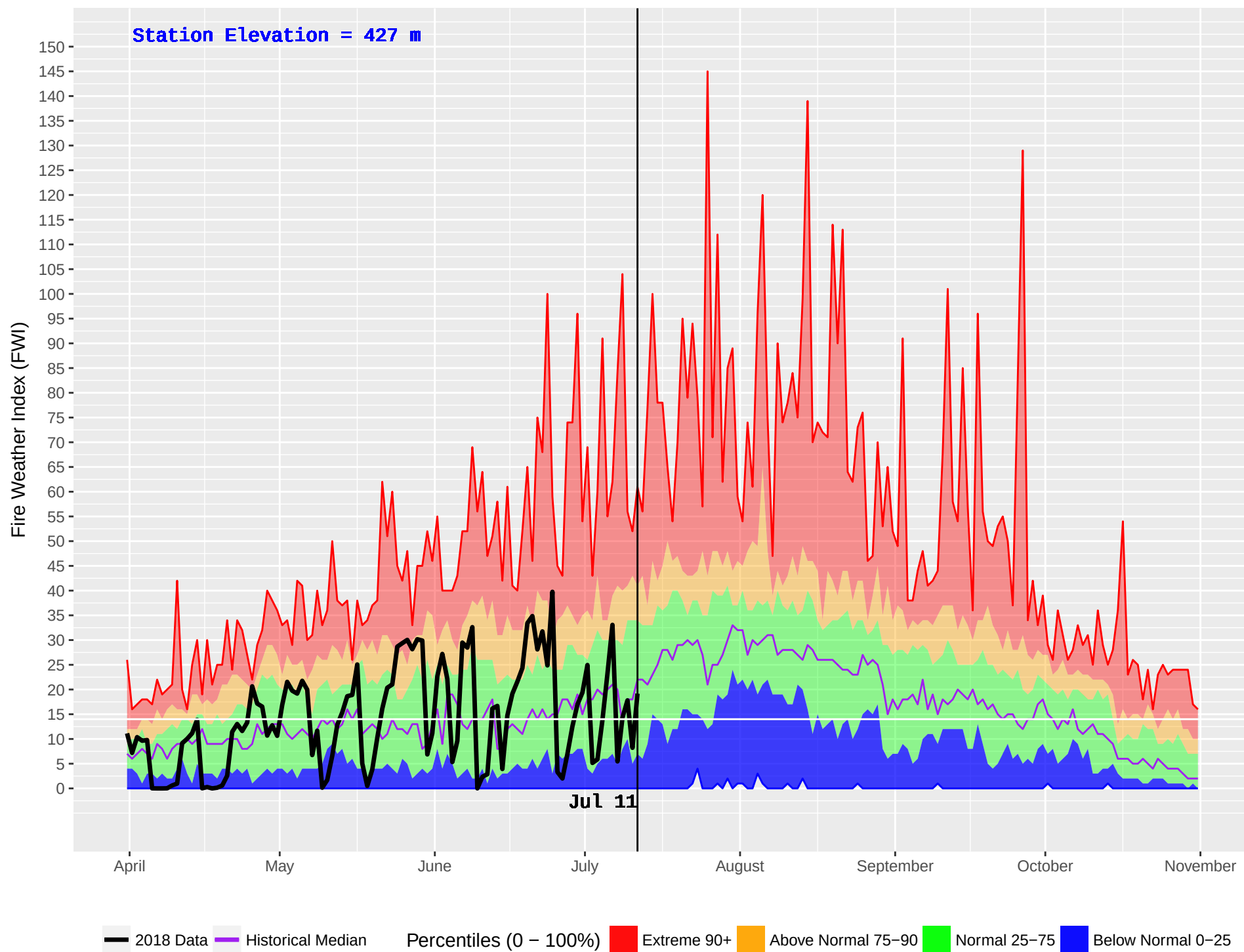
PENTICTON RS (328) : Historical (1970–2016) and Current (2018) Noon Fire Weather Index (FWI)
