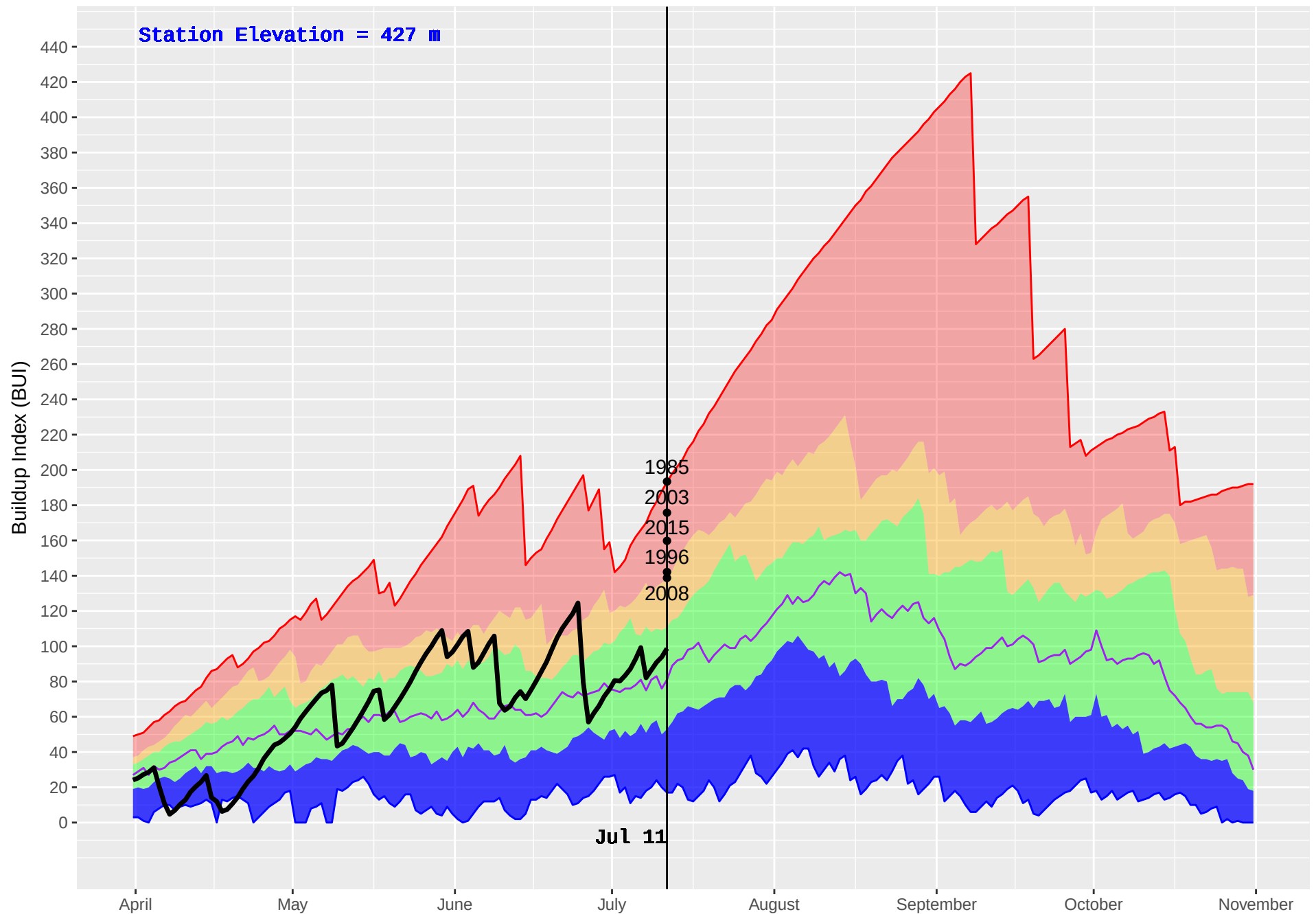
PENTICTON RS (328) : Historical (1970–2016) and Current (2018) Noon Buildup Index (BUI)
