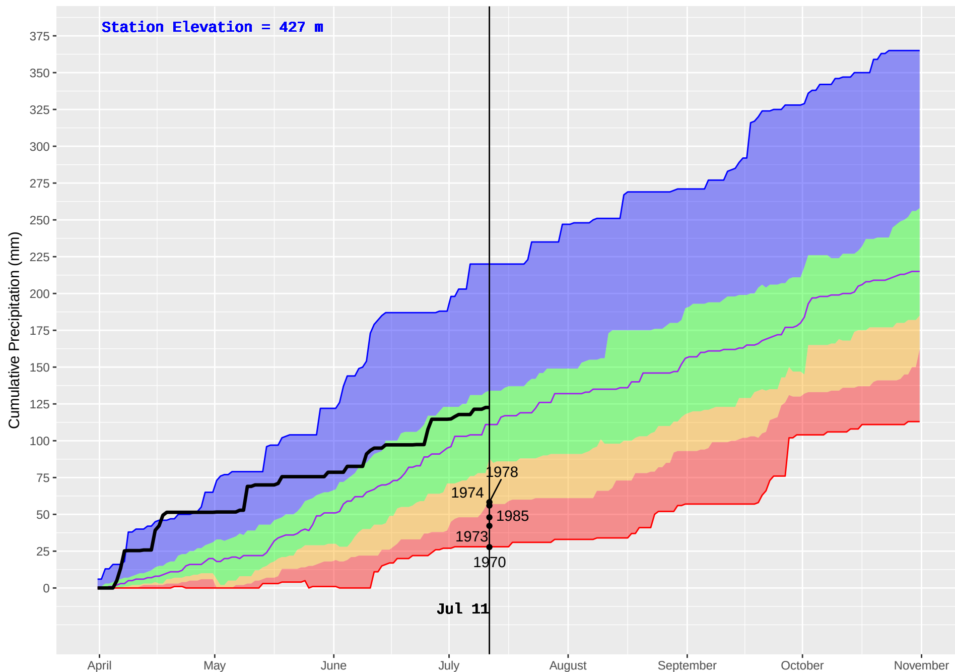
PENTICTON RS (328) : Historical (1970–2016) and Current (2018) Noon Cumulative Precipitation
